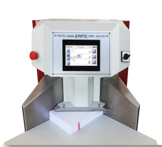
NEW DESIGN WITH POWERFUL CLAMP
