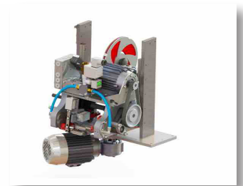
ADR 32 COUNTING HEAD AT 3000 SHEETS/MIN
